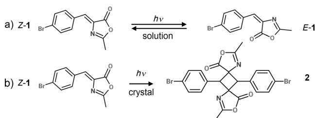
Scheme 1. a) Solution photoisomerization and b) solid-state photodimerization.
